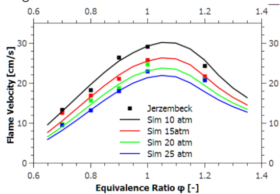
Predicted and measured laminar flame speeds for PRF 87 / air at 373 K and different ambient pressures. Experiments from Jerzembek et al 2009.
